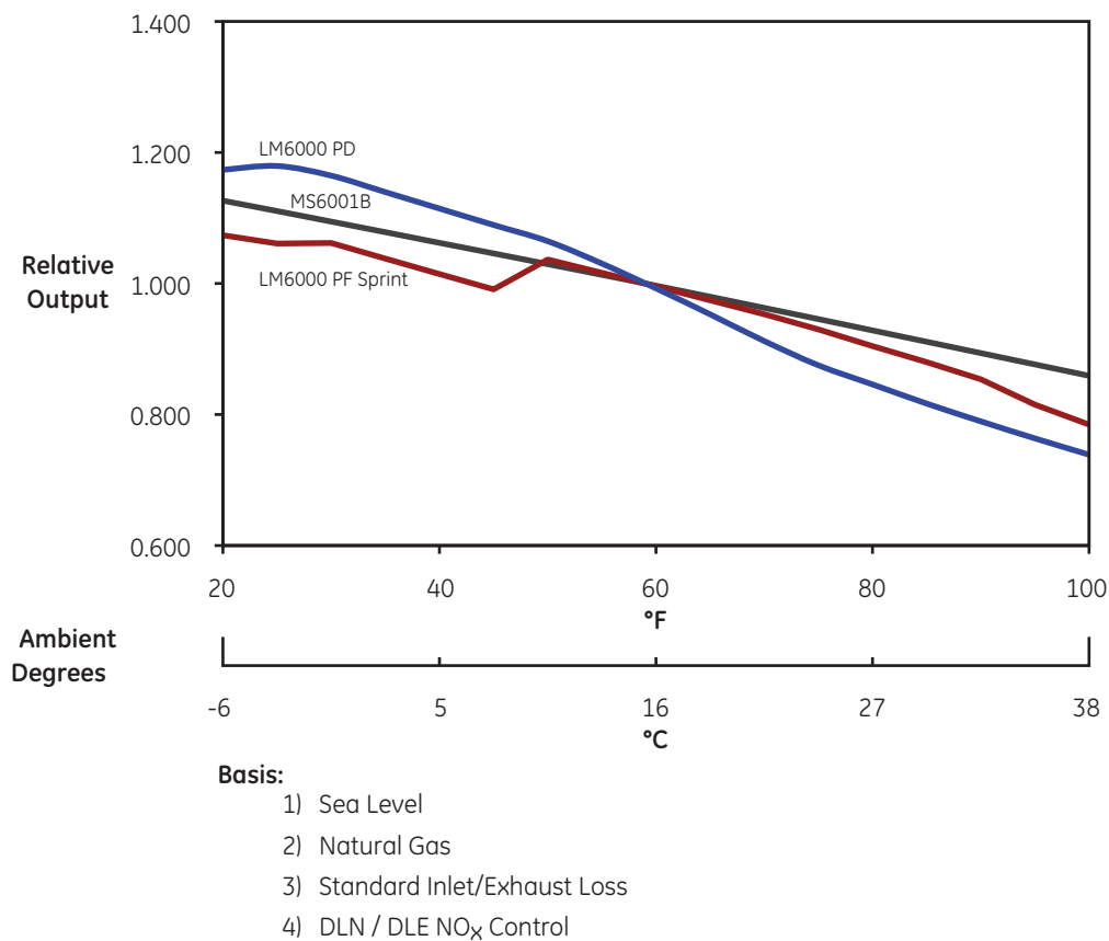
Figure 15. Gas turbine ambient output characteristics
